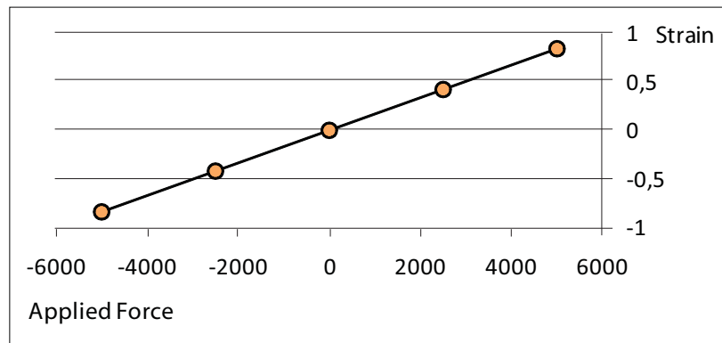
Figure 6: Force Strain Relation
